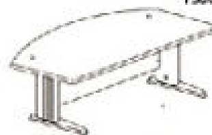
EXECUTIVE TABLE TT 180A 1800W x 900D x 745H
